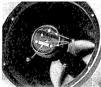
Collimation Adjusting Screws (A) Secondary mirror housing (B) Collimation adjusting screws (C) Schmidt corrector plate (D) Serial Number
