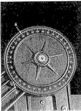
Reading the Dec. Setting Circle
