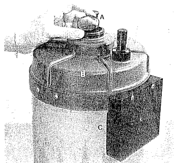
Series VI Filters & Tripod Adapter (A) Series VI filter (B) Rear cell (C) C8 photo tripod adapter
