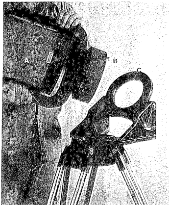
Mounting Your Celestron on the Wedge (A) Telescope (B) Bolt, partially threaded into the drive base (C) Wedge slot
