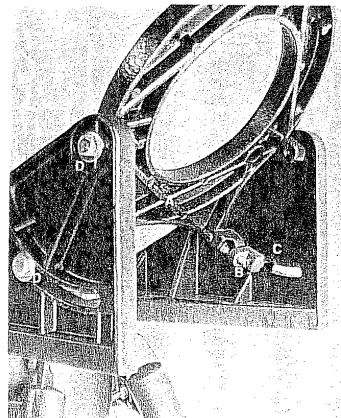
Adjusting the Wedge (A) Tilt plate (B) Adjusting screw (C) Latitude adjuster (D) Tilt plate bolts (on both sides of wedge)
