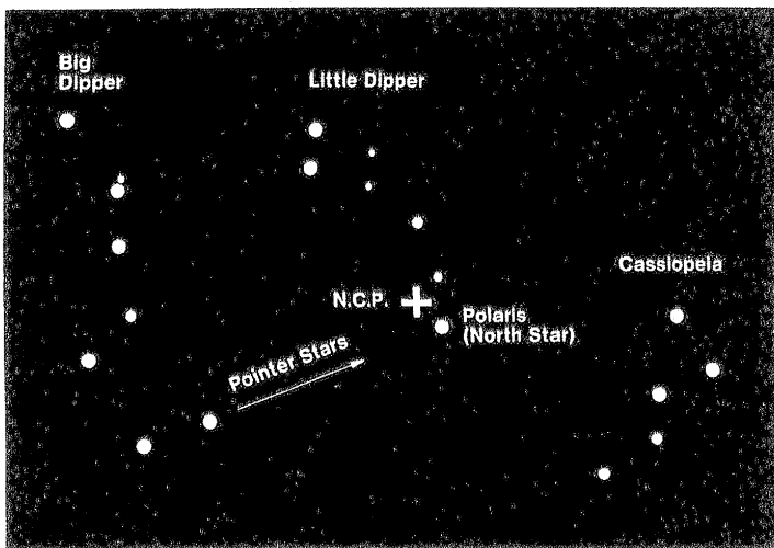
The Celestial Polar Region
