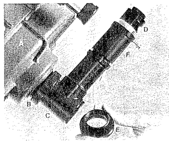
The Off-Axis Guiding System (A) Rear cell (B) Slip ring (C) Guider body (D) Illuminated reticle ocular. Also shown is the tele-compressor (E) and its eyepiece extender (F).
