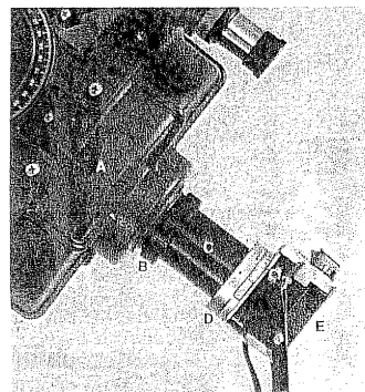
The T-Adapter (A) Rear cell (B) Slip ring (C) T-adapter (D) T-ring (E) Camera body
