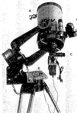
Astrophotography with the C8 (A) C8 counterweights (B) 35mm camera with lens on the piggyback mount (C) Off-axis guiding system (D) Cold camera (E) Drive corrector
